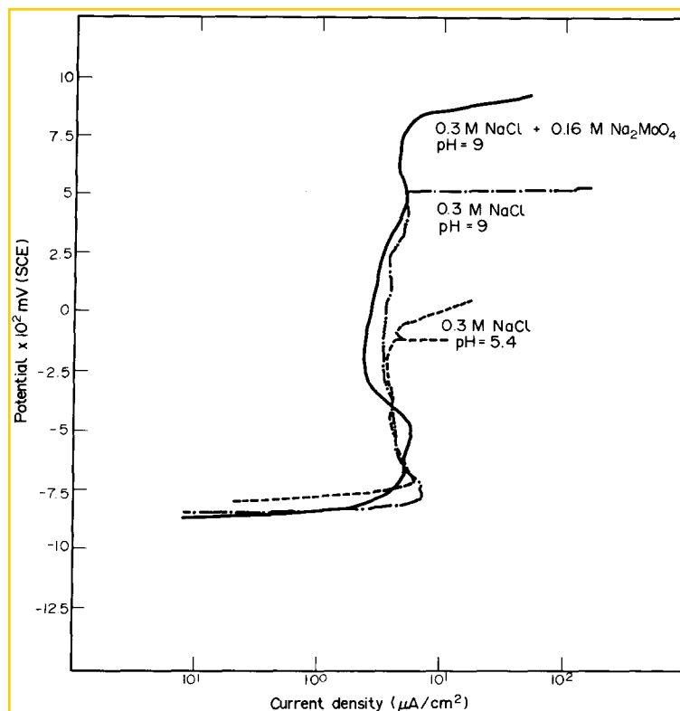
FIG. 1. Polarization diagrams for Fe-19Cr-9Ni alloy obtained in de-aerated 0.3 M NaCl (pH 5.4), 0.3 M NaCl (pH 9.0) and 0.3 M NaCl + 0.16 M \text{Na}_2\text{MoO}_4 (pH 9.0).
